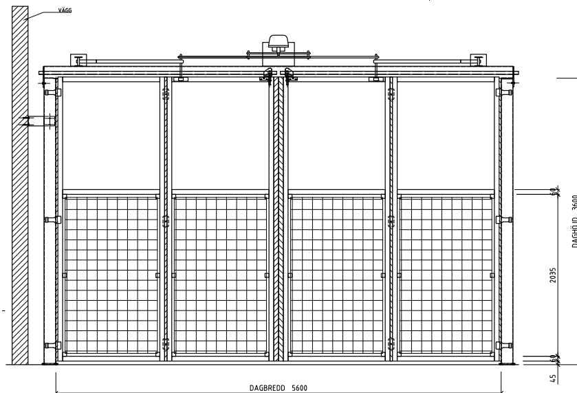
4 section folding door with electric operation, viewed from the machine side.
