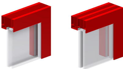
Cut in glazed wall section EI-60
