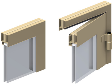
Cut in glazed wall section
